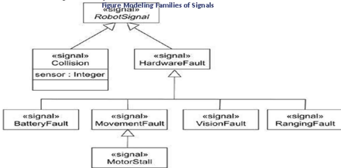
Modeling Exceptions
