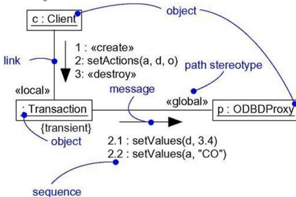
Figure Collaboration Diagram
